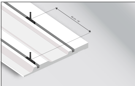
1. Put the T clips on the baseboard/skirting board backside staggered between the different grooves, leaving a space of 40 cm/16" between them.
