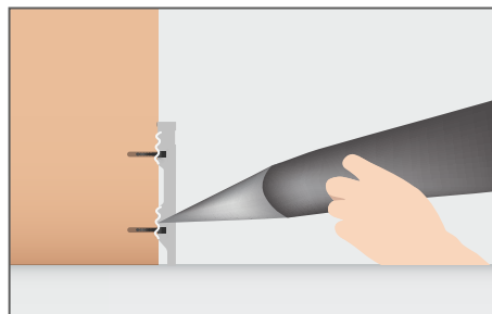
5. Complement the installation with a moderate amount of adhesive. For a better mounting, add adhesive or neutral silicone to the profile backside.
